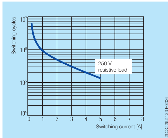
Contact lifetime
